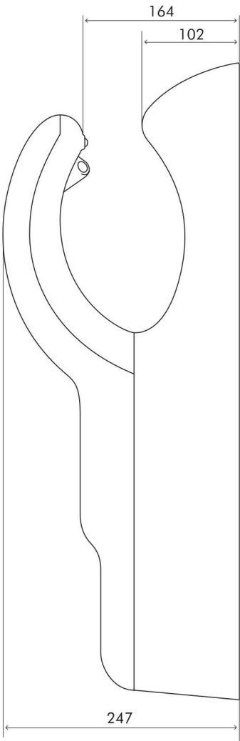
SIDE ELEVATION
