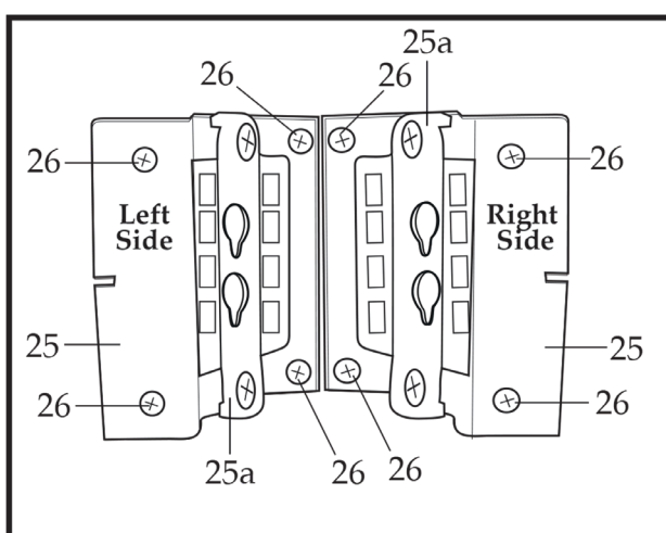
Looking into unit with back cover off at cup support locking assemblies.
